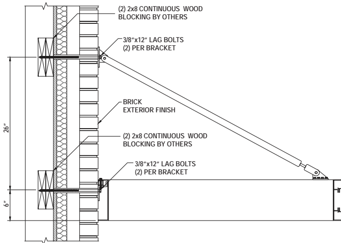
BRICK WITH INSULATION OVER WOOD BLOCKING
