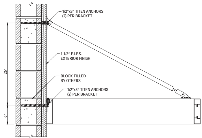
E.F.I.S. OVER CMU BLOCK WALL
