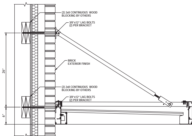
BRICK WITH INSULATION OVER WOOD BLOCKING
